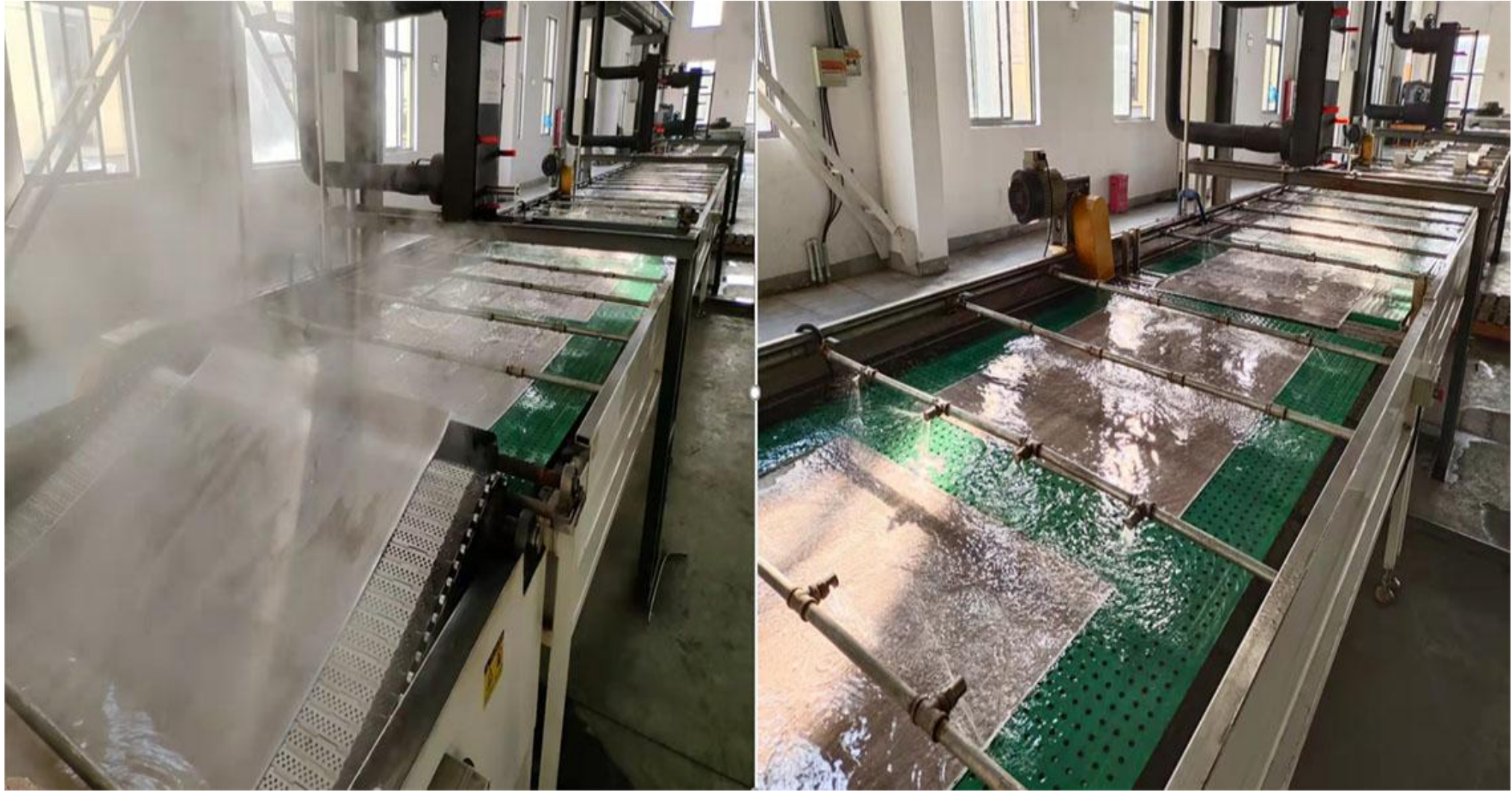
Annealing+UV coating/ Laminated LVT(Japan equipment)
